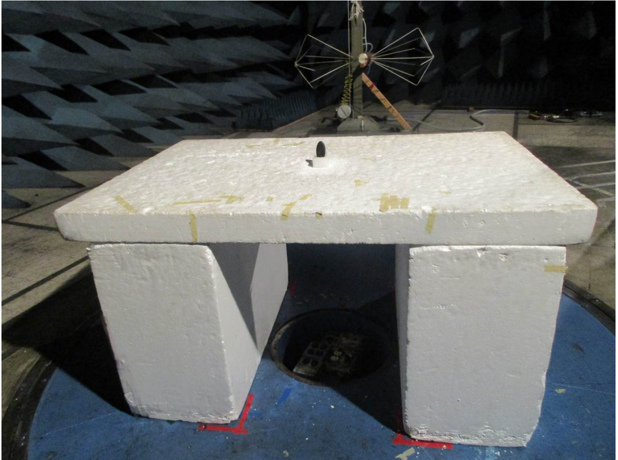
Figure 3: Radiated Emissions – Back View – 30 MHz – 200 MHz – Standing
