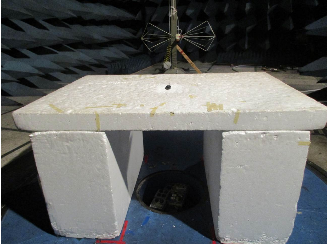
Figure 15: Radiated Emissions – Back View – 30 MHz – 200 MHz – Flat
