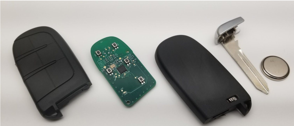
CDSSL-G000 Internal Photos - TOP
