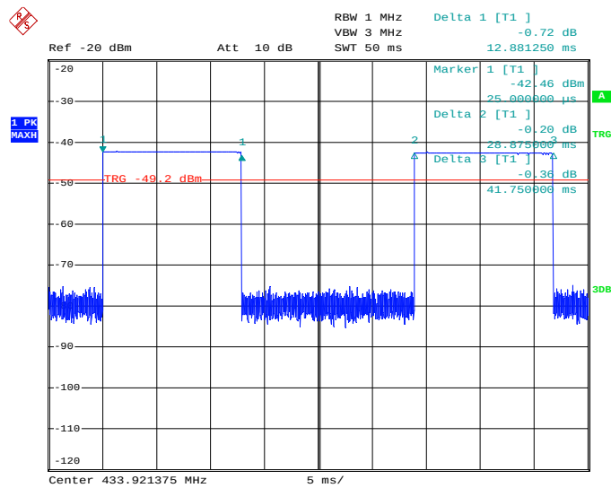
Figure 7.4.2-4: Periodic Operation – 5 Seconds – FSK 14 kHz Modulation
