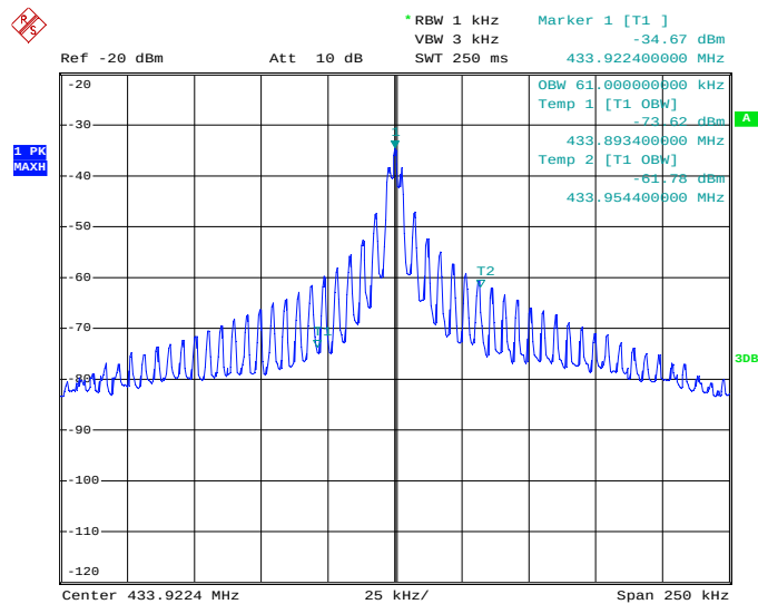
Figure 7.2.2-1: 20dB Bandwidth – ASK
