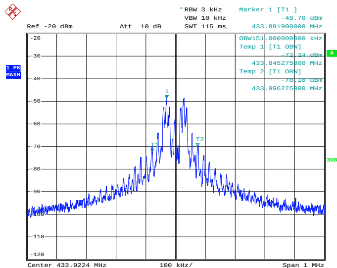
Figure 7.2.2-3: 20dB Bandwidth – FSK1 14 kHz Deviation
