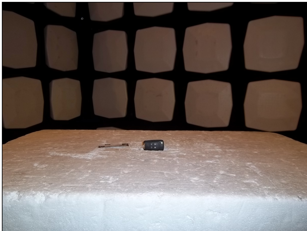
Figure 4: Radiated Emissions – XPOS
