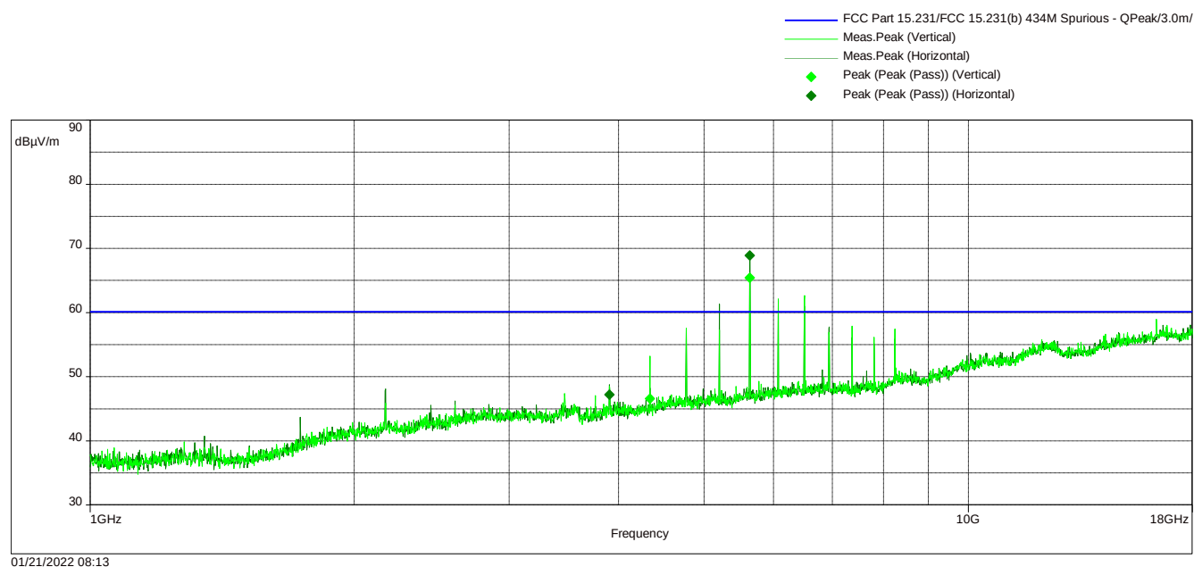
Figure 2-26 – RE Spurious Emissions 1-18 GHz – FSK, High Channel
