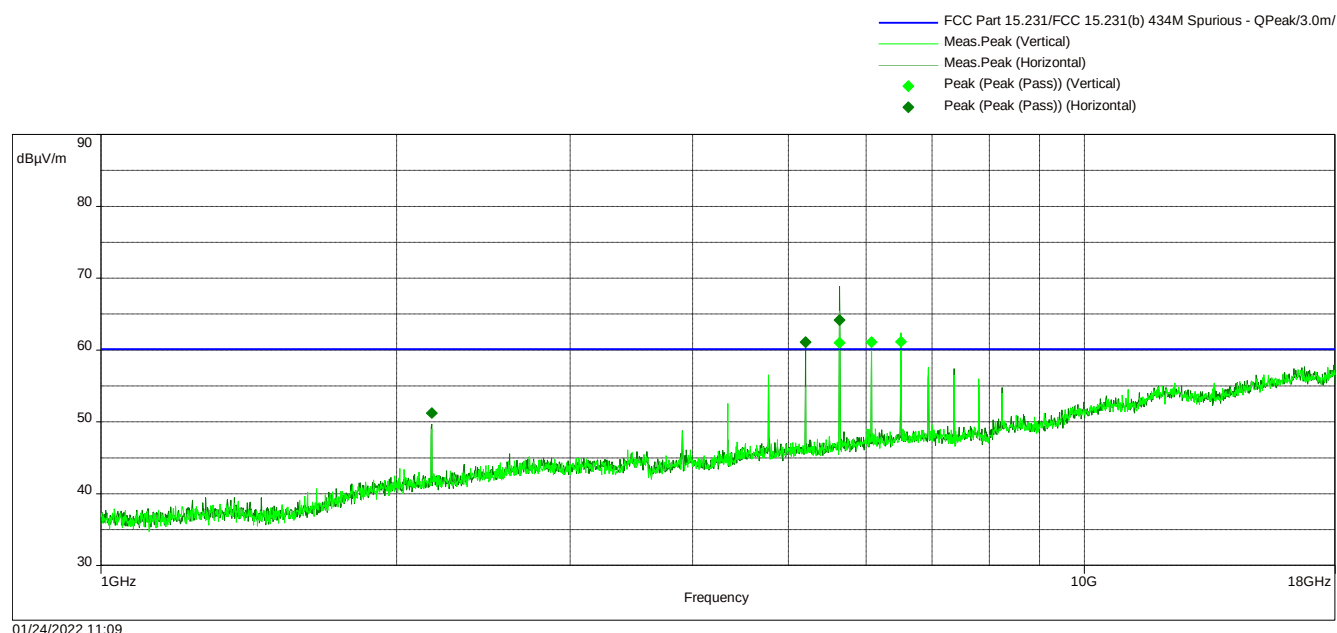
Figure 2-24 – RE Spurious Emissions 1-18 GHz – ASK, High Channel
