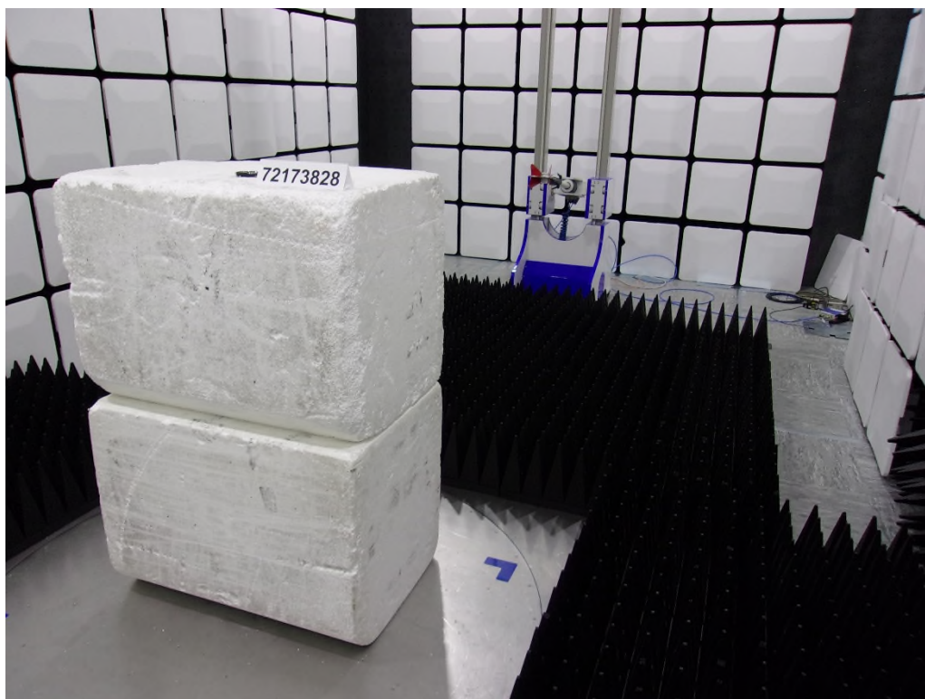
Photo 1.3-3 – RE Spurious Emissions 1-18 GHz, Front, Worst-case Orientation
