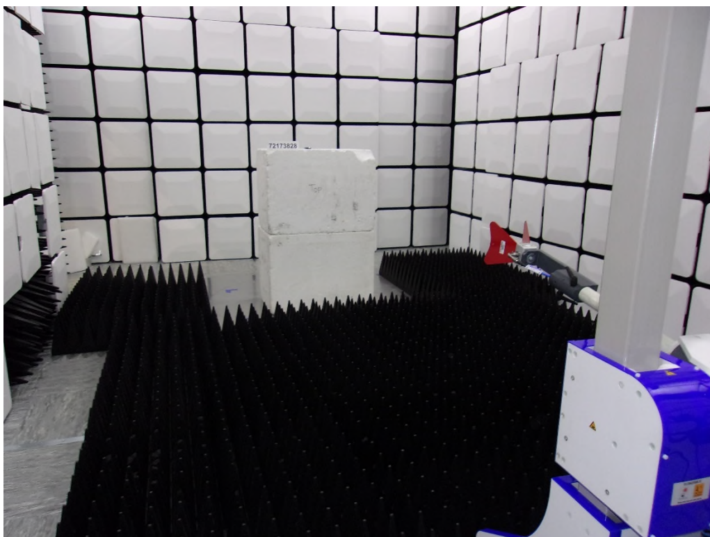
Photo 1.3-4 – RE Spurious Emissions 1-18 GHz, Rear, Worst-case Orientation
