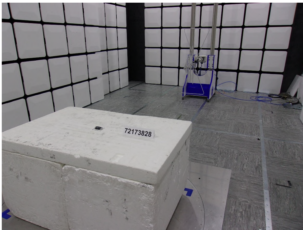
Photo 1.3-1 – RE Spurious Emissions 30-1000 MHz, Front, Worst-case Orientation
