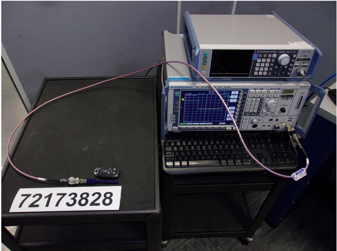
Photo 1.2-2 – Conducted Measurements, 2
