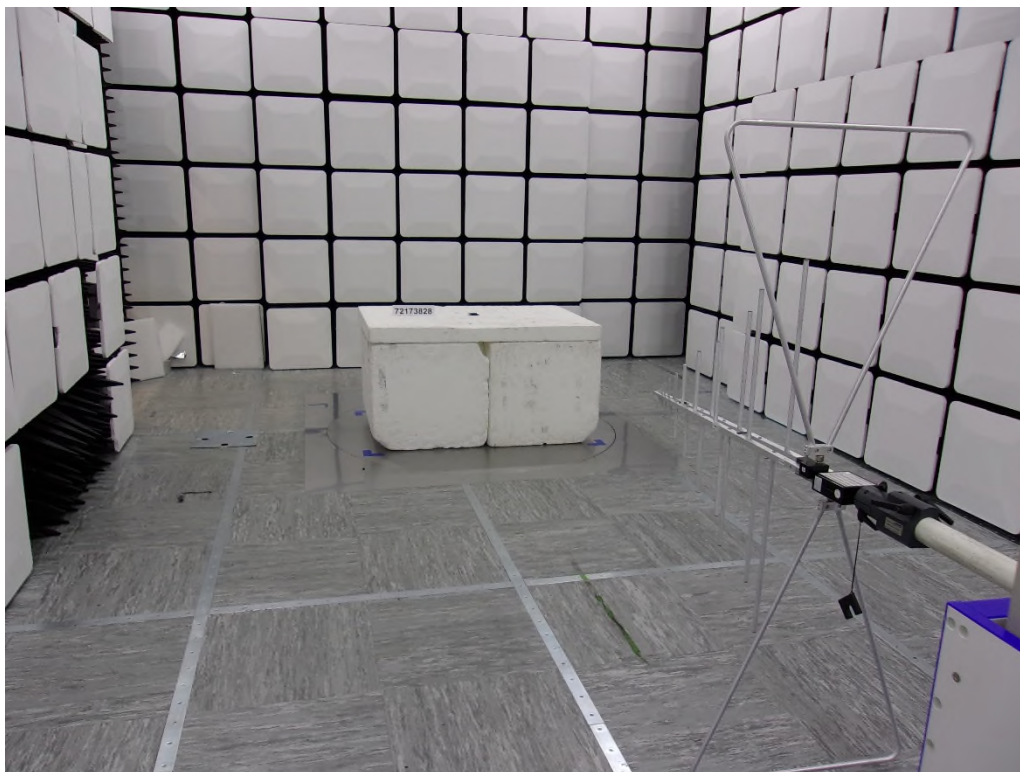
Photo 1.3-2 – RE Spurious Emissions 30-1000 MHz, Rear, Worst-case Orientation
