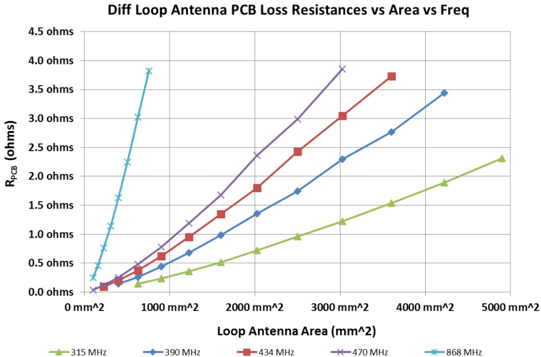
Figure 2. Dielectric Loss Resistance R_{PCB} vs. Area vs. Frequency
