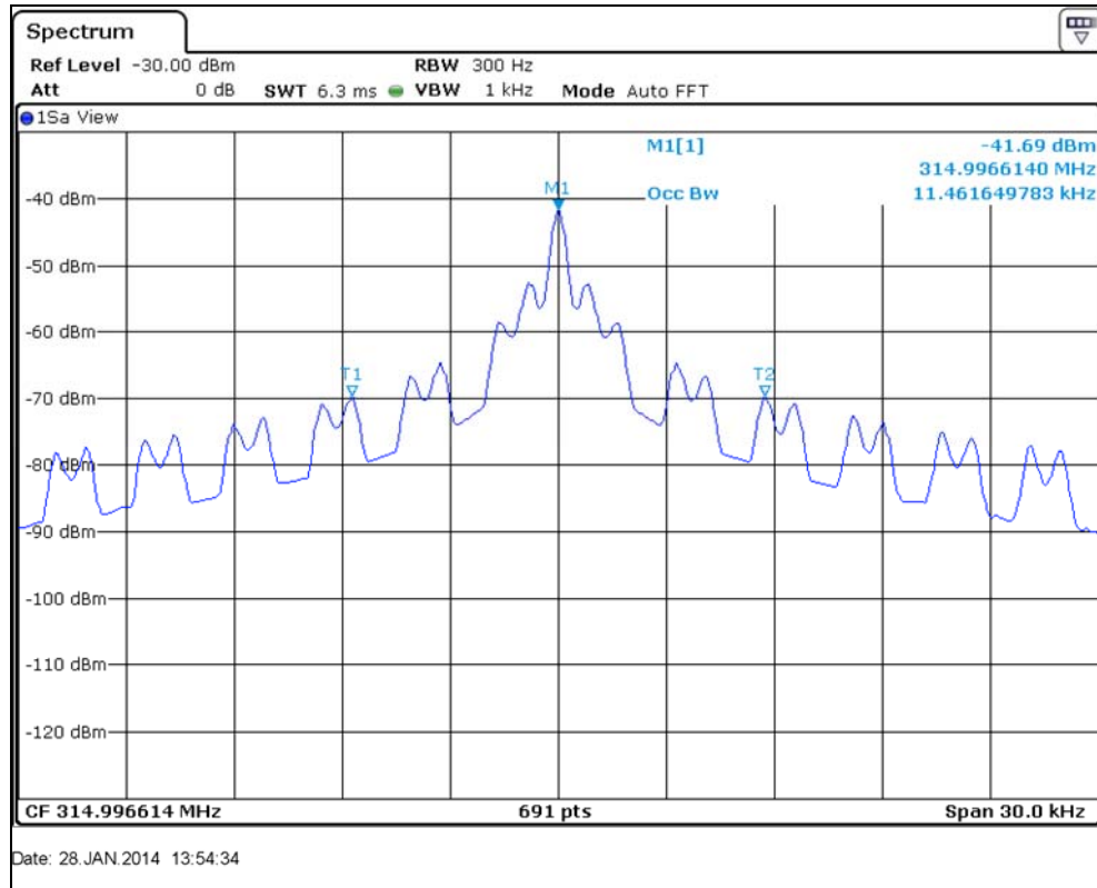
Figure 7.4.2-2: 99% Occupied Bandwidth
