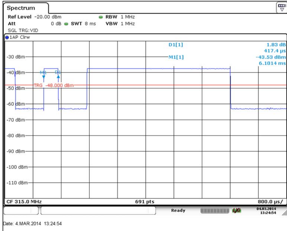
Figure 7.5.2-4: Duty Cycle –Pulse Width (T1)
