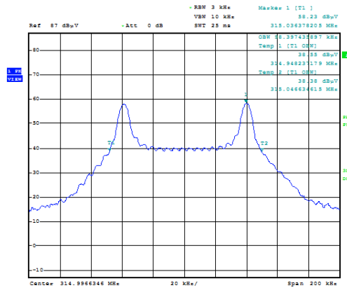
Figure 7.4.2-4: 99% Occupied Bandwidth – 315 MHz
