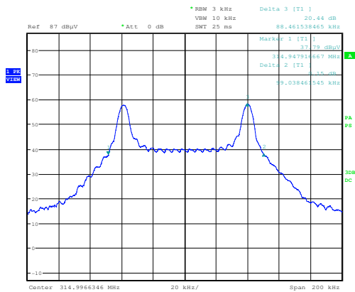
Figure 7.4.2-3: 20 dB Bandwidth – 315 MHz
