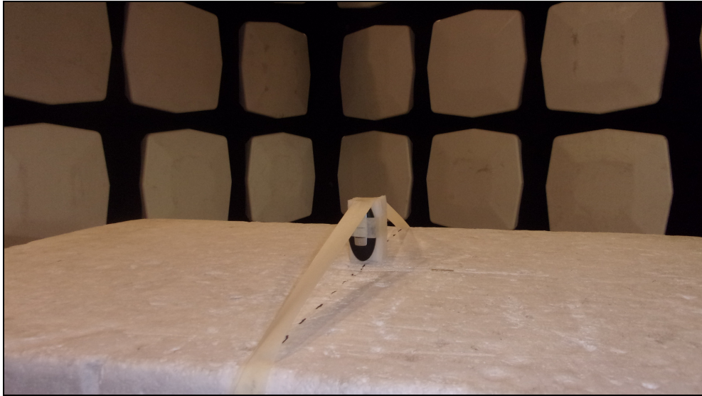
Figure 5: Radiated Emissions – YPOS
