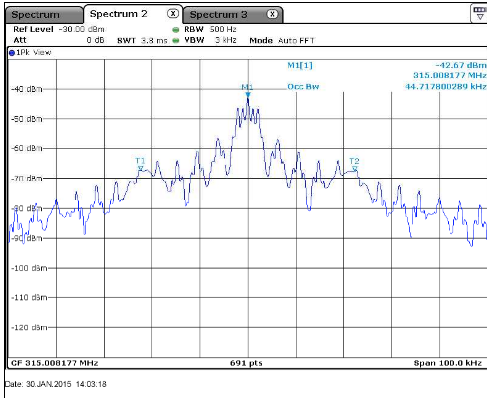
Figure 7.4.2-2: 99% Occupied Bandwidth
