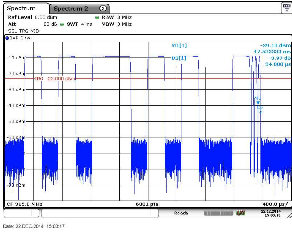
Figure 7.5.2-5: Duty Cycle – Pulse Width (T3)
