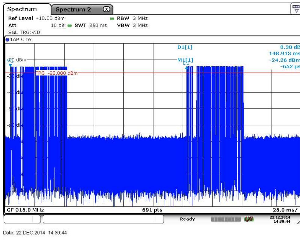
Figure 7.5.2-1: Duty Cycle
