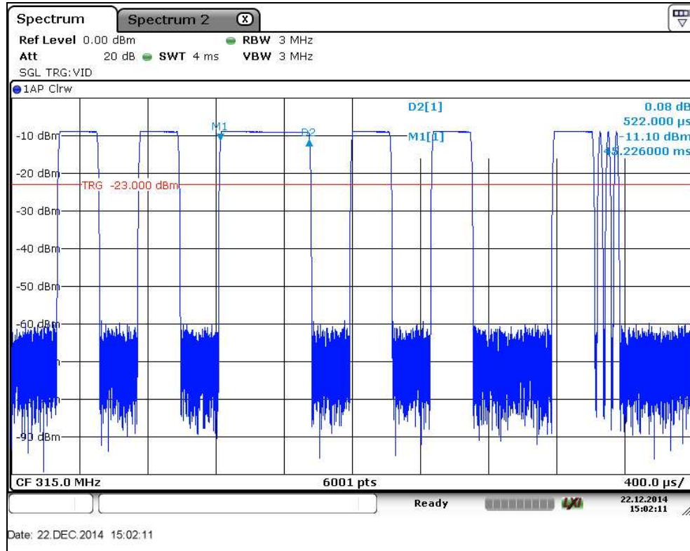
Figure 7.5.2-4: Duty Cycle – Pulse Width (T2)
