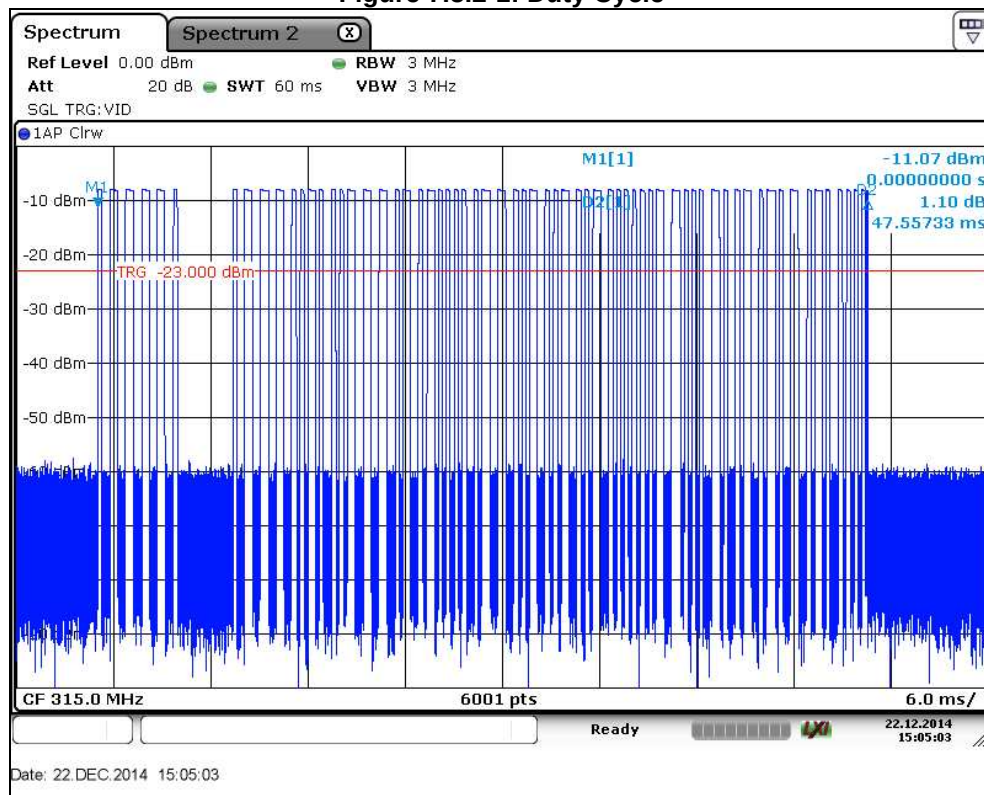
Figure 7.5.2-2: Duty Cycle
