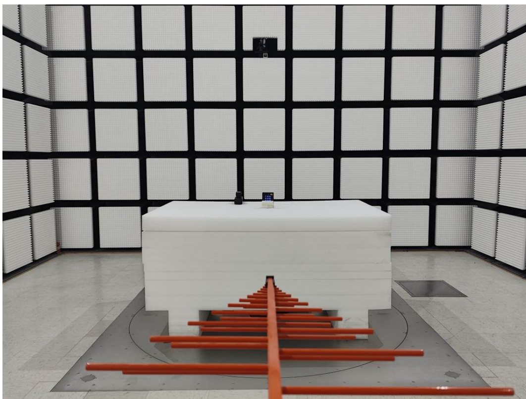
Radiated Emission 30M-1GHz View MW-322
