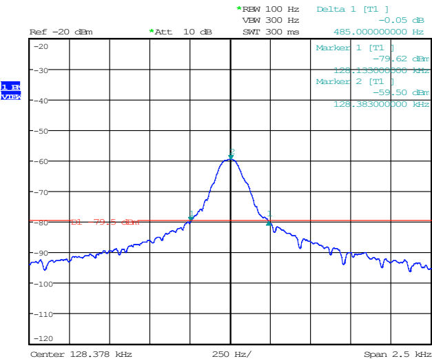
Standby Mode / Simultaneous Charge and Discharge with iPhone
