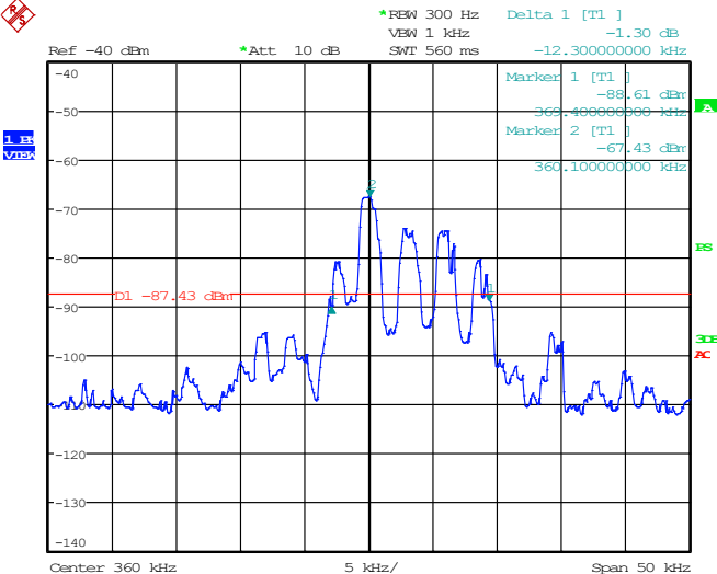
Charging with iPhone (15W)
