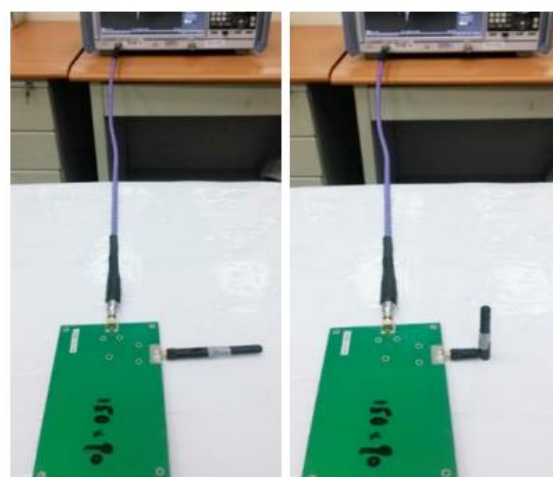
Antenna straight
