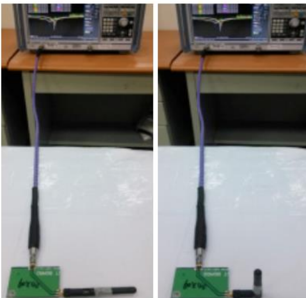
Antenna straight
