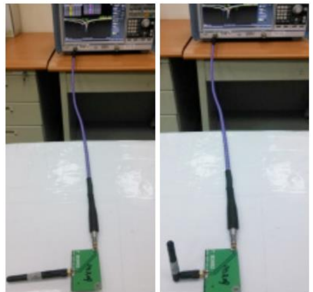
Antenna straight
