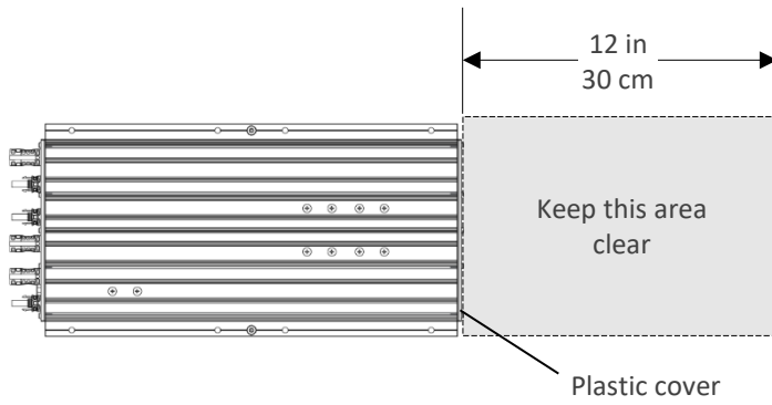
Figure 6: Keep this area of the String Optimizer clear to improve radio signal
