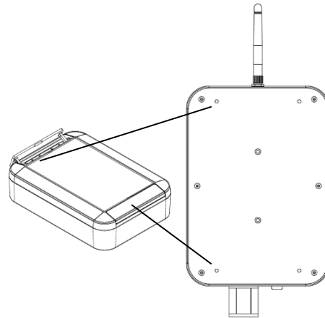
Figure 8: Mounting holes behind the blind lid on the front of the Ampt CU
