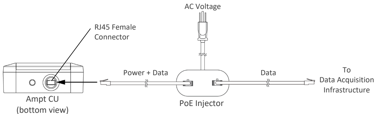
Figure 11: Generic Power over Ethernet (PoE) connection diagram – follow the instructions for your device
