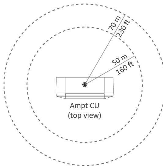
Figure 5: Top view of the Ampt CU with radio signal ranges (Ampt CU not to scale)
