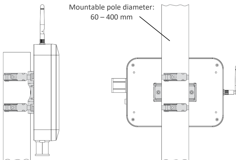
Figure 9: Mounting examples that minimize obstructions
