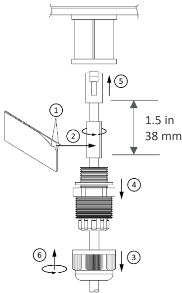
Figure 10: Connecting the Ethernet cable
