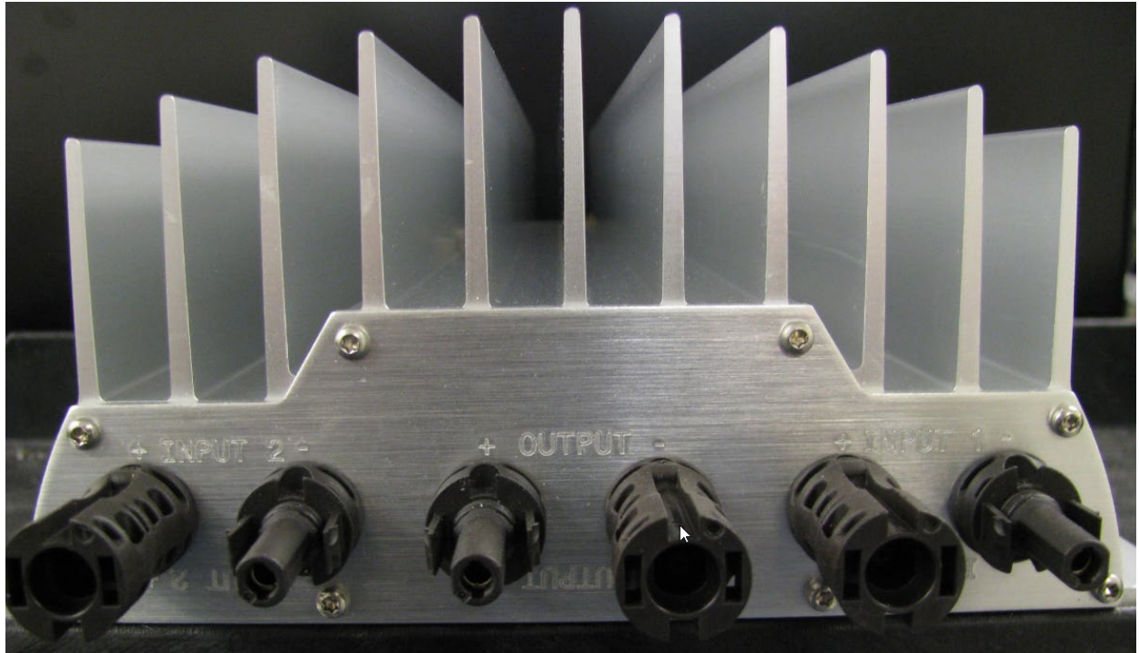
Unit Side 1 (front)
