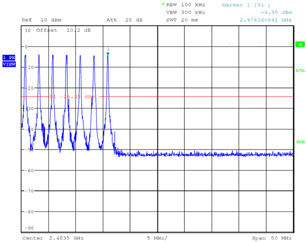
Plot 6.7 Conducted Band Edge, High Channel (Hopping)
