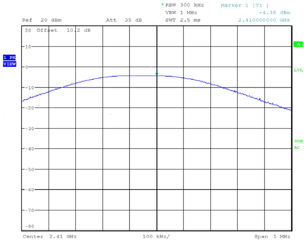
Plot 2.1– Output Power Low Channel
