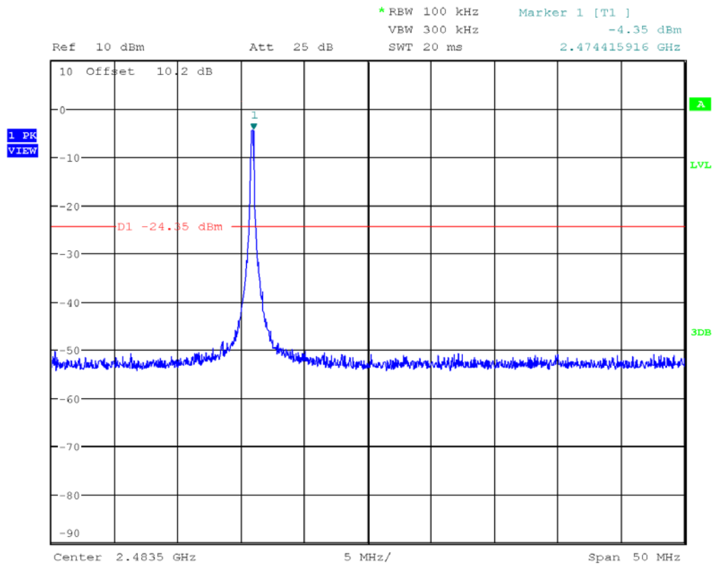
Plot 6.6 Conducted Band Edge, High Channel
