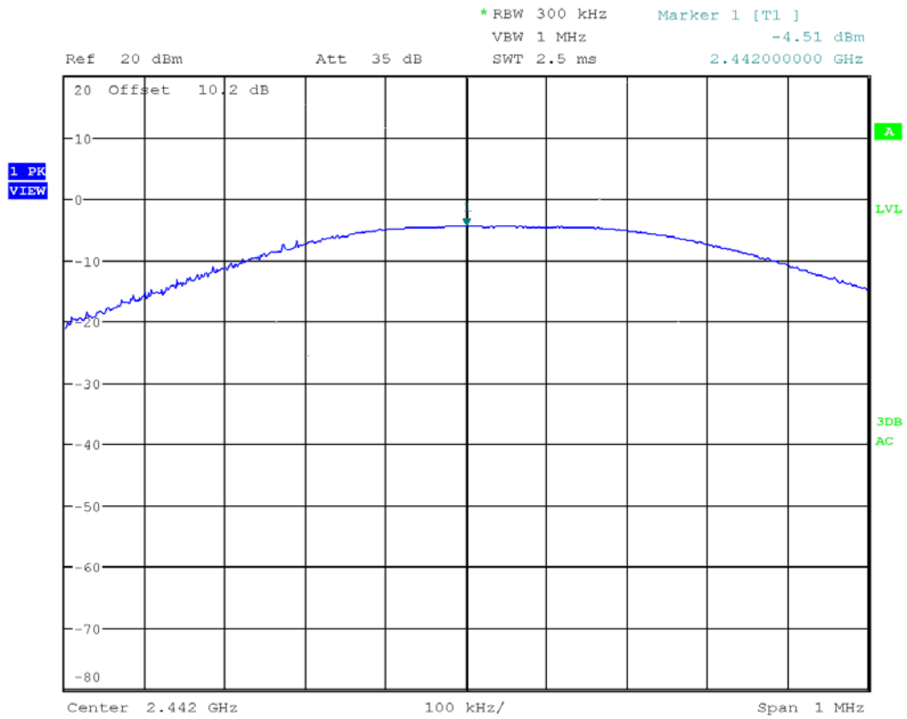
Plot 2.2 – Output Power Middle Channel
