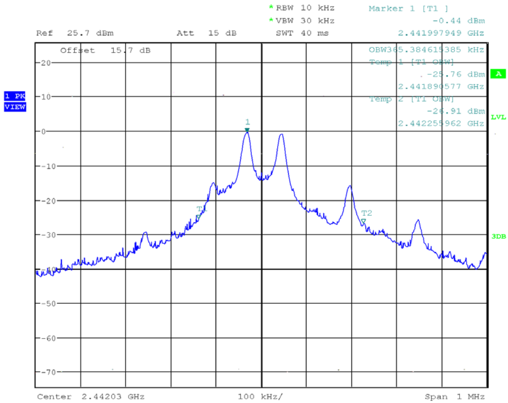
Plot 1.4 – 99% Bandwidth Middle Channel
