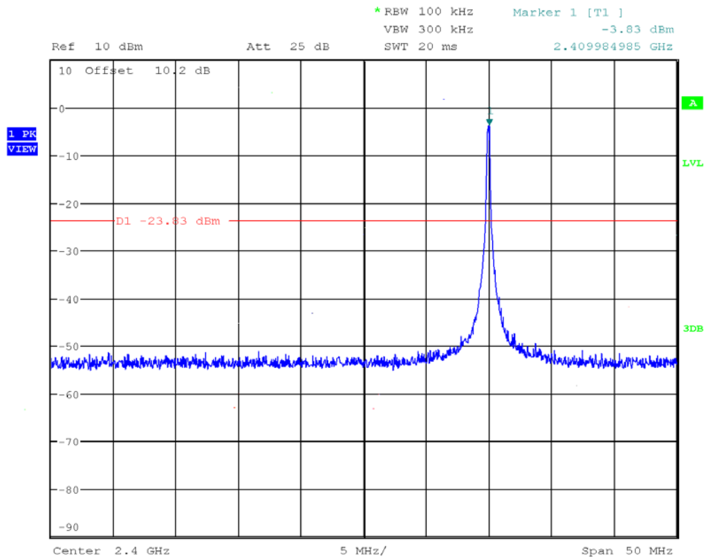
Plot 6.4 Conducted Band Edge, Low Channel
