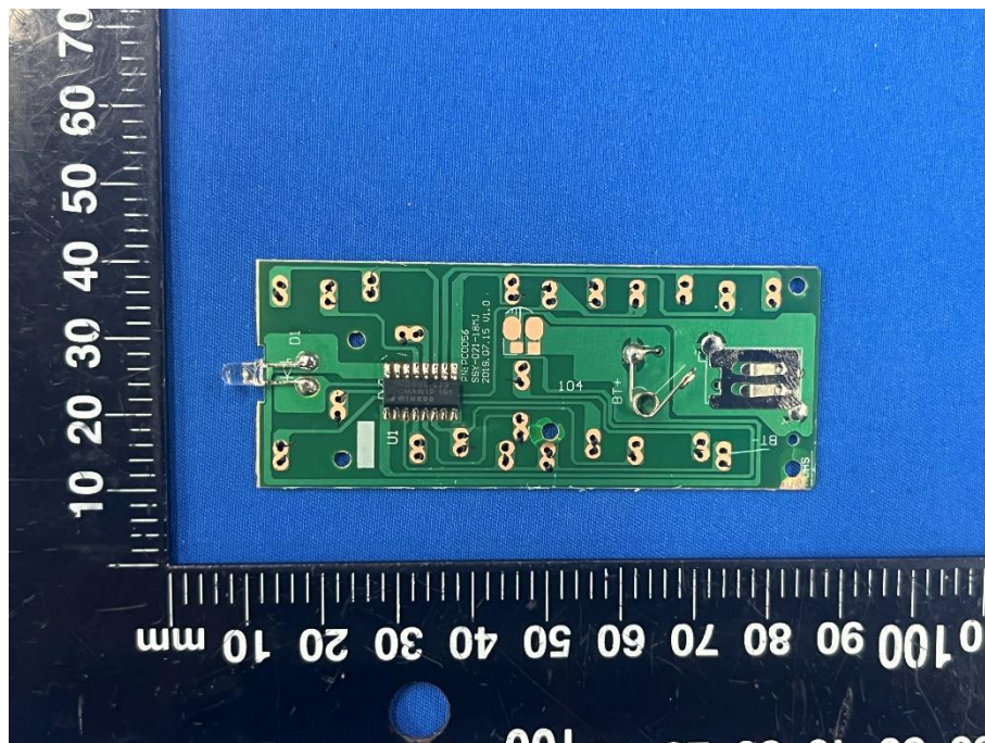
MAIN BOARD TOP VIEW (REMOTE CONTROL)
