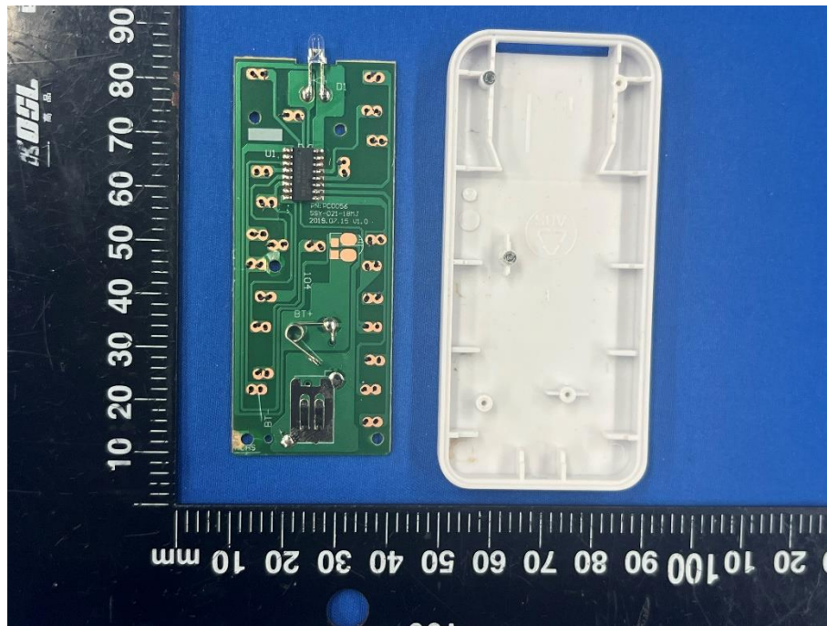
EUT UNCOVER VIEW 4 (REMOTE CONTROL)
