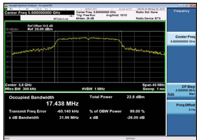
U-NII-2c 99% Bandwidth-802.11a(20MHz) ,5600MHz
