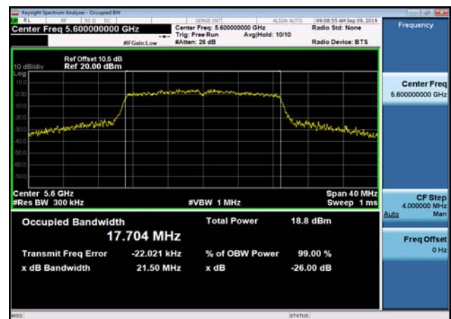
U-NII-2c 99% Bandwidth-802.11n(20MHz) ,5600MHz
