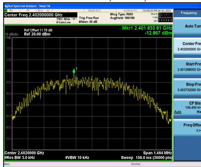
Mode 1 CH00(2402MHz)
