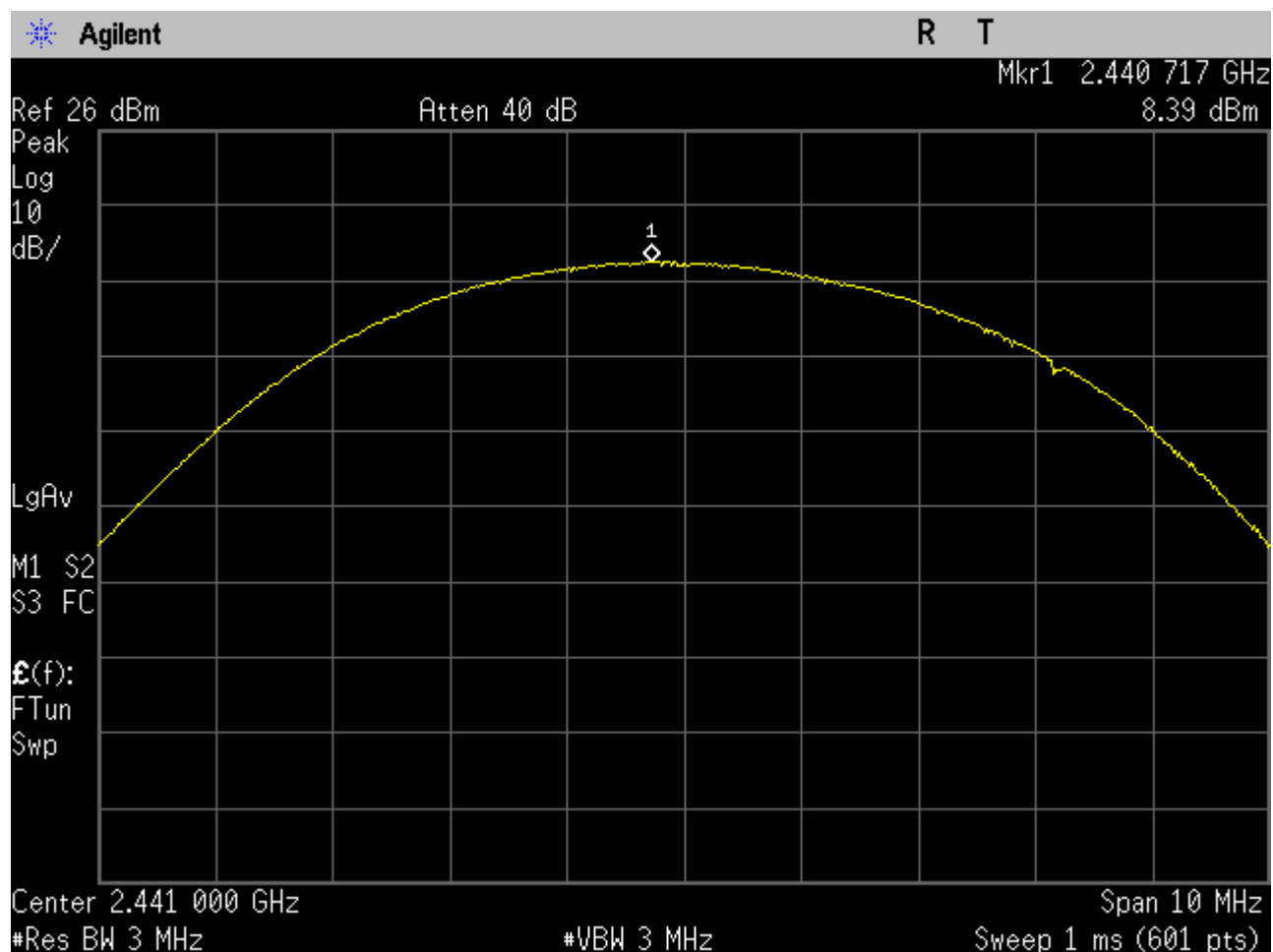
Figure 2: Conducted Output Power, Mode B
