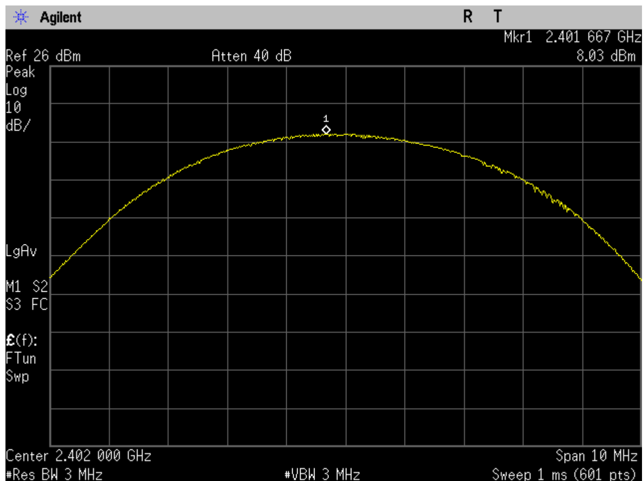
Figure 1: Conducted Output Power, Mode A
