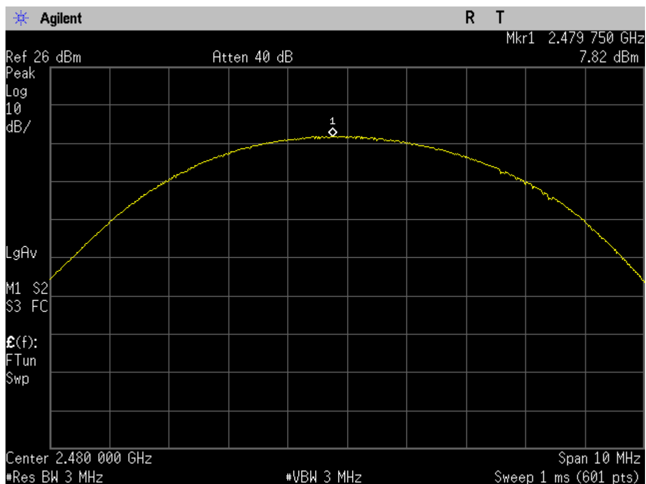
Figure 3: Conducted Output Power, Mode C
