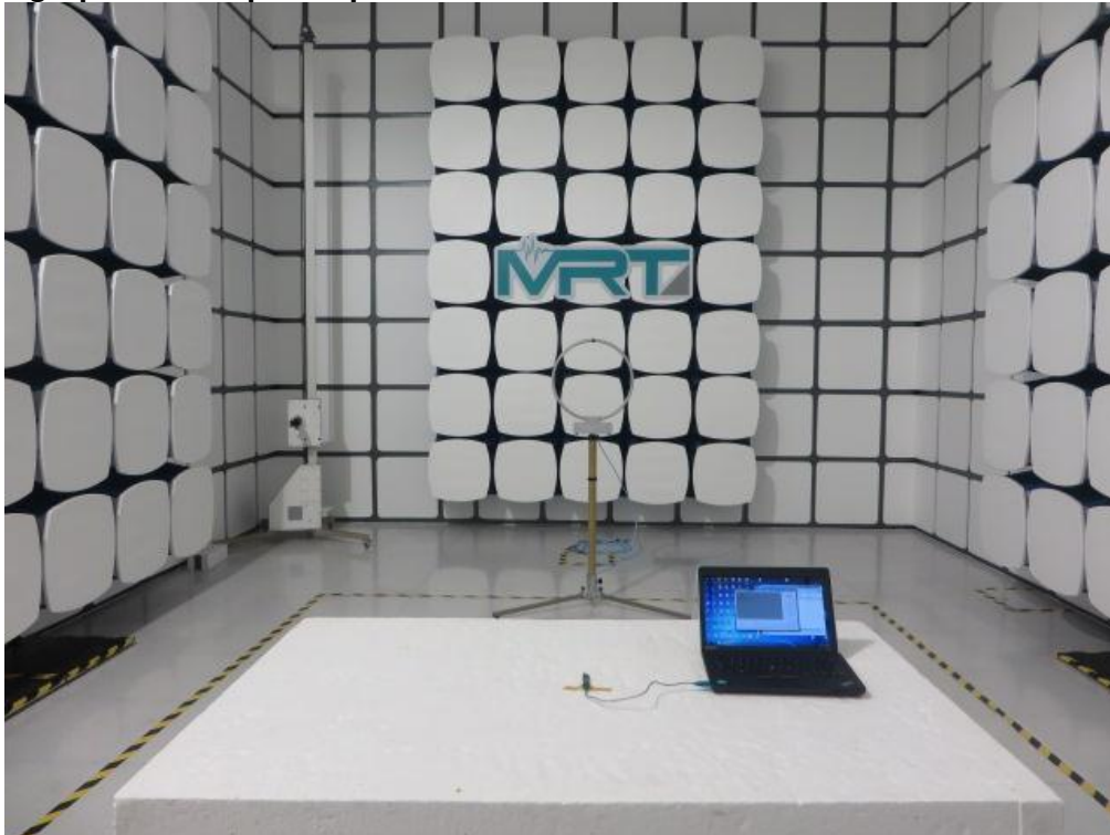
Photograph 3: Set-up for Spurious Emissions below 1GHz
