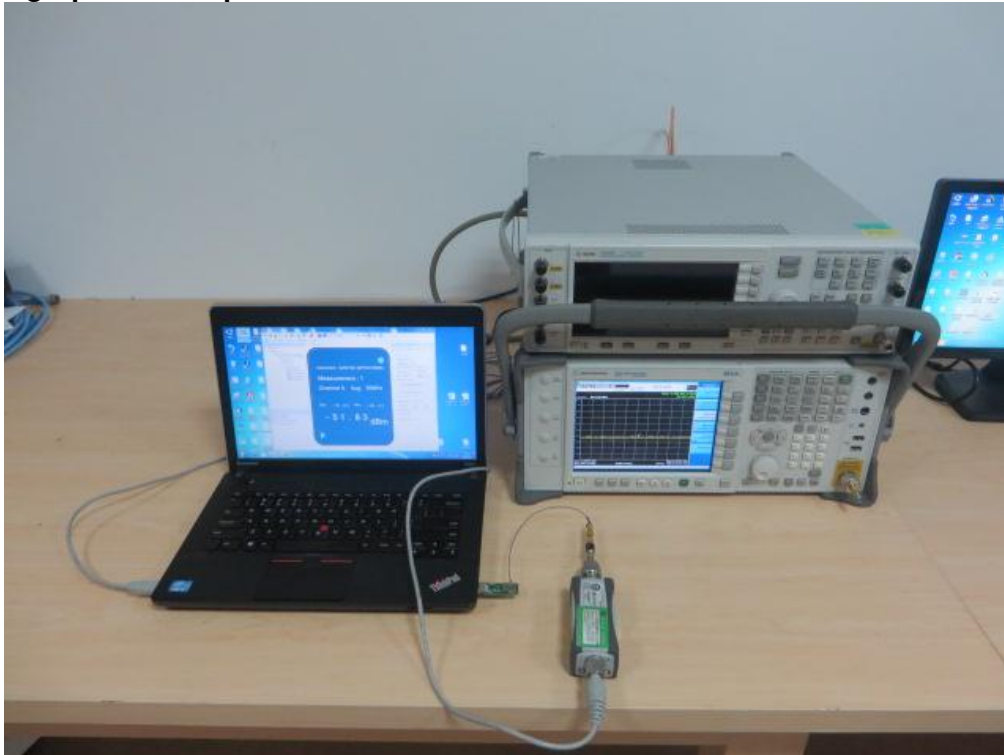
Photograph 2: Set-up for Conducted RF test at Antenna Port
