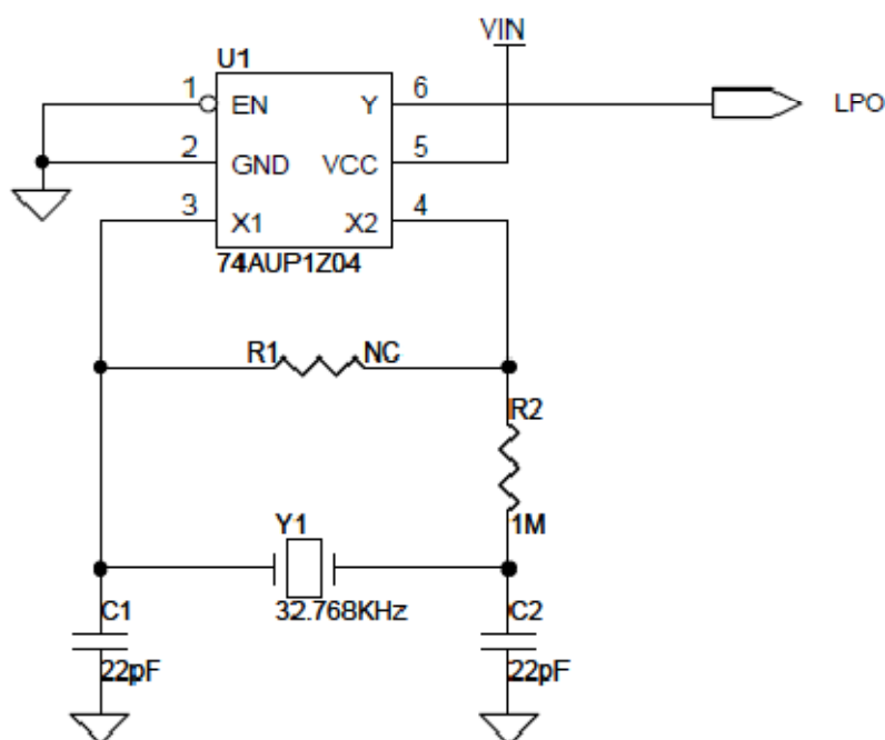
External LPO Reference Circuit
