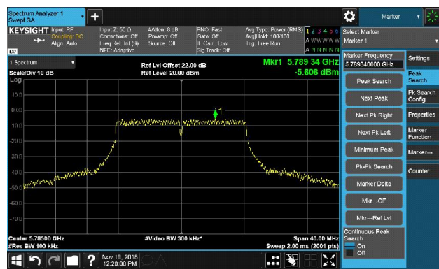
Channel 157 (5785MHz)
