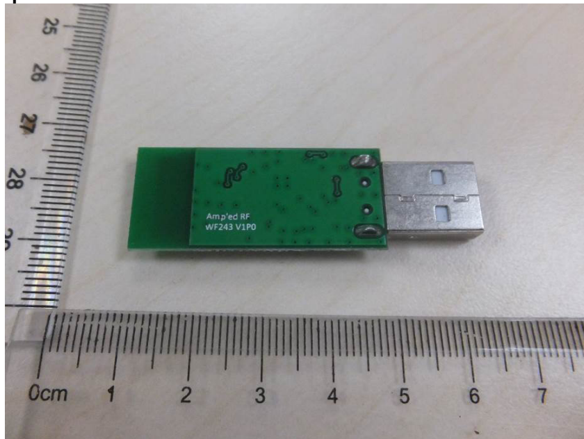
Photograph 2: Rear view of the EUT
