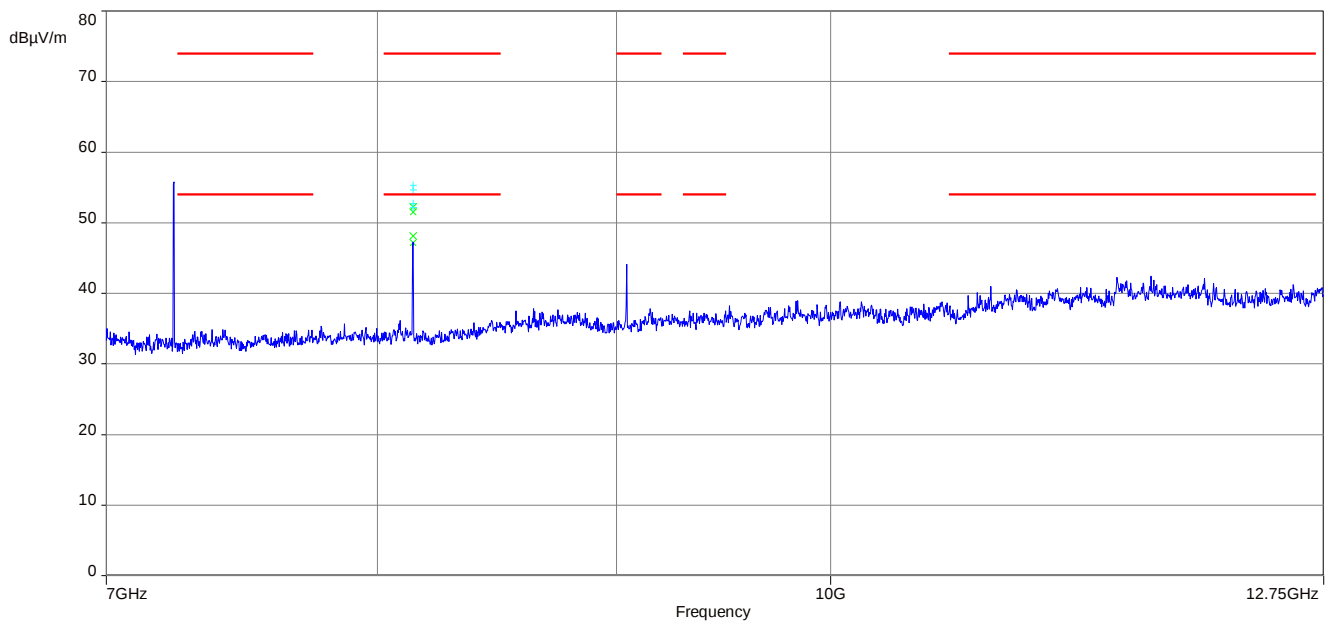
Plot 1: 7 GHz –12.75 GHz, horizontal & vertical polarisation (lowest channel)
