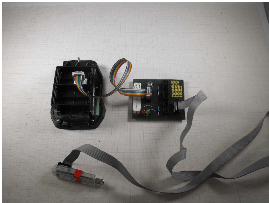
Photo 2: Battery cover removed
