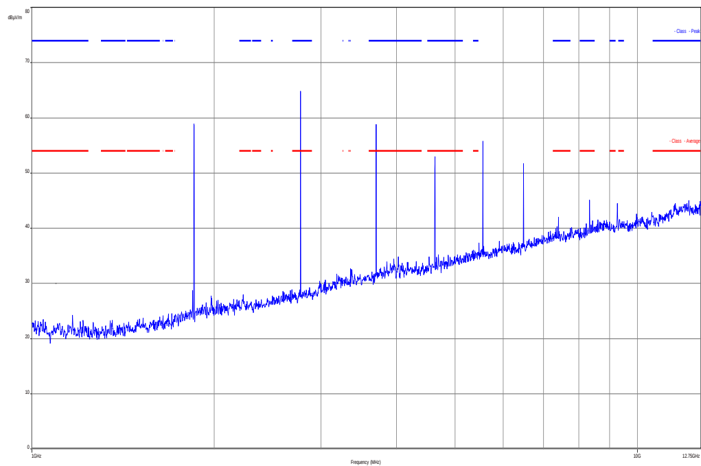
Plot 6: 1 GHz – 12.75 GHz, horizontal &amp; vertical polarisation (highest channel)
