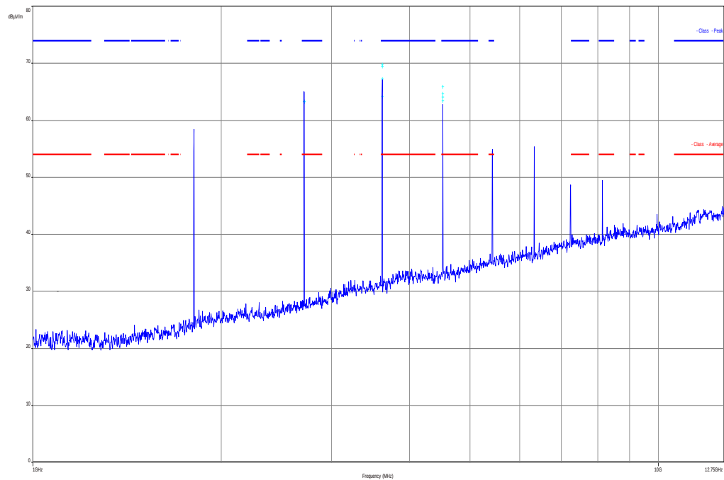
Plot 2: 1 GHz – 12.75 GHz, horizontal &amp; vertical polarisation (lowest channel)
