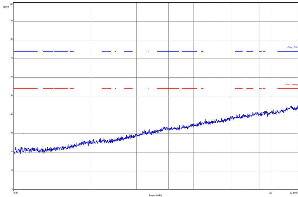
Plot 2: 1GHz – 12.75 GHz, RX-Mode, horizontal &amp; vertical polarisation
