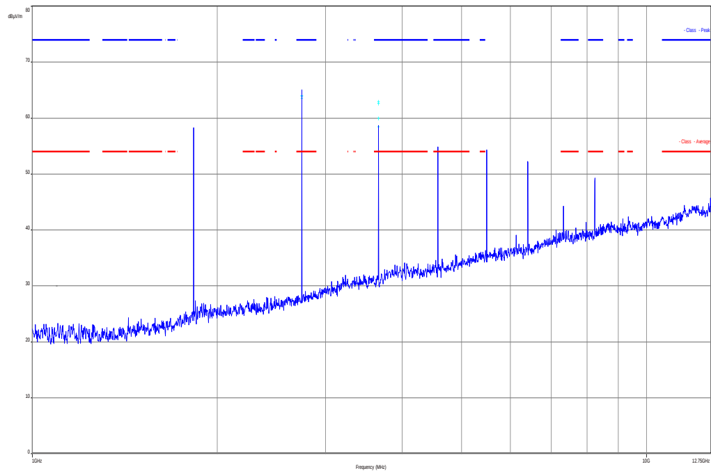
Plot 4: 1 GHz – 12.75 GHz, horizontal &amp; vertical polarisation (middle channel)
