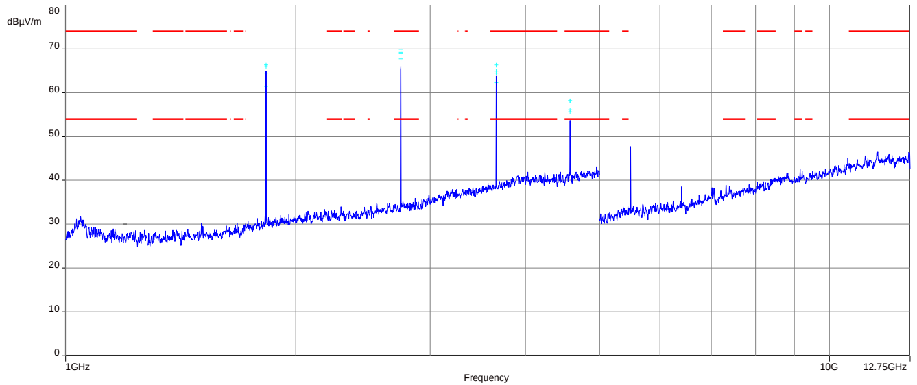
Plot 4: 1 GHz – 12.75 GHz, horizontal &amp; vertical polarisation (middle channel)
