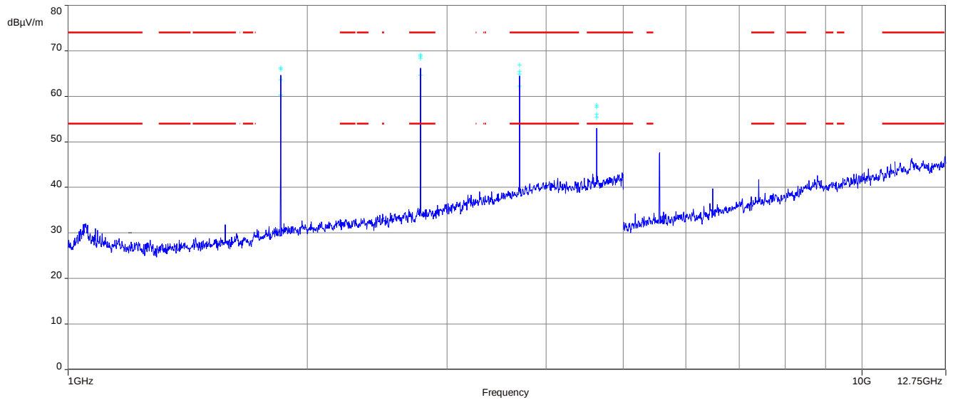
Plot 6: 1 GHz – 12.75 GHz, horizontal &amp; vertical polarisation (highest channel)
