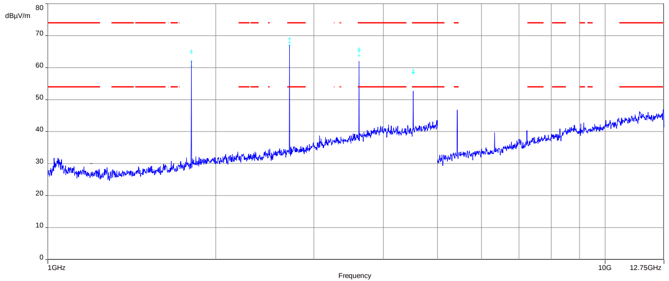
Plot 2: 1 GHz – 12.75 GHz, horizontal &amp; vertical polarisation (lowest channel)
