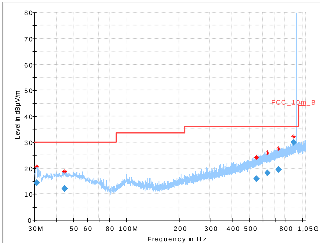
Plot 3: 30 MHz – 1 GHz, horizontal &amp; vertical polarization (highest channel)
