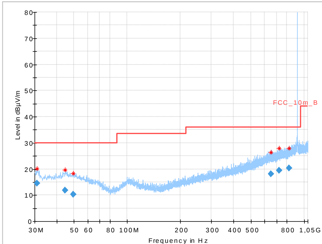
Plot 2: 30 MHz – 1 GHz, horizontal &amp; vertical polarization (middle channel)
