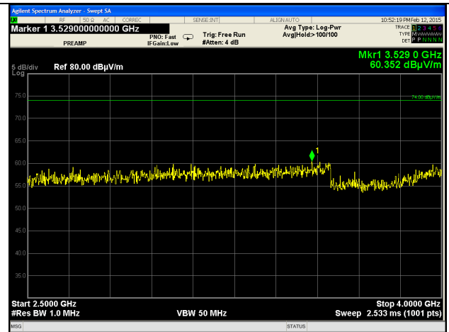
2.5-4 GHz - Peak
