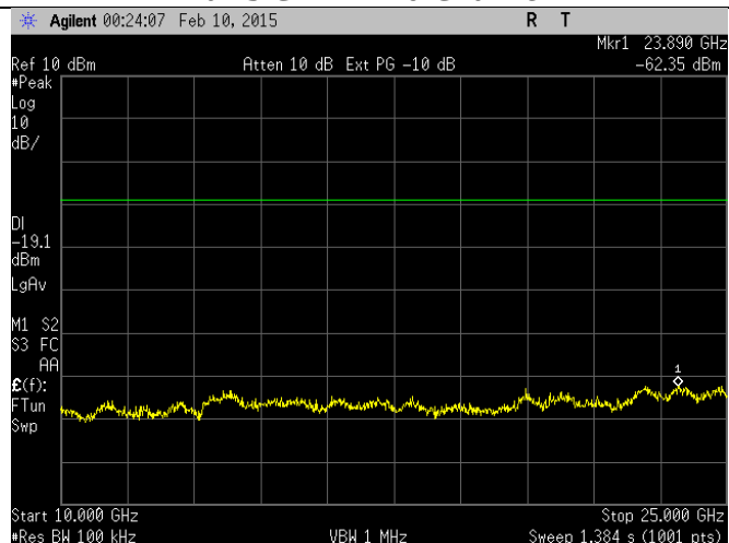
10-25 GHz – High Channel
