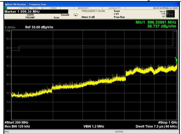
200-1000 MHz - Horizontal Polarity
