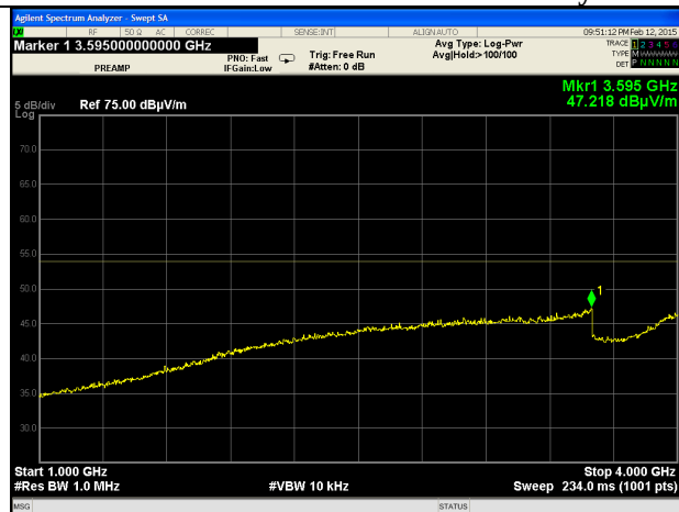
1-4 GHz - Horizontal Polarity - Average
