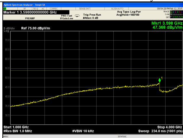
1-4 GHz - Vertical Polarity - Average
