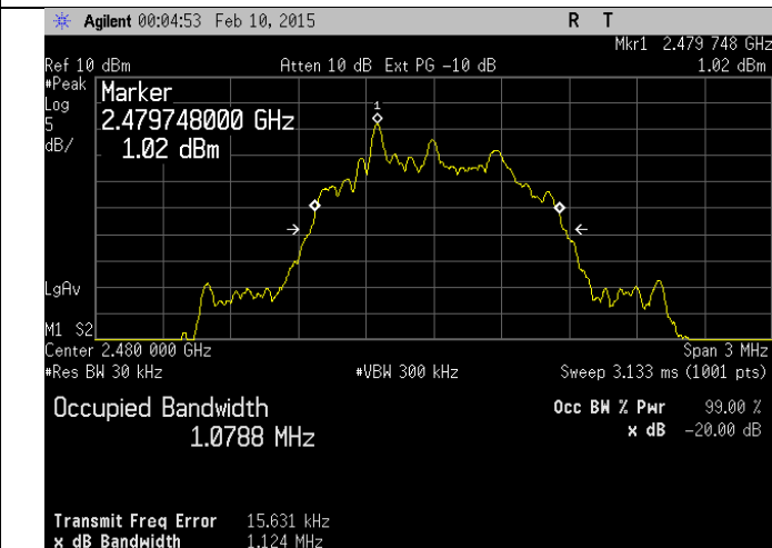
OBW + 99% BW – High Channel
