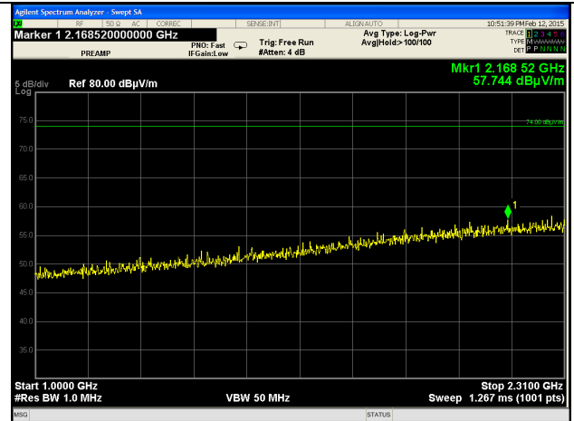
1-2.31 GHz - Peak
