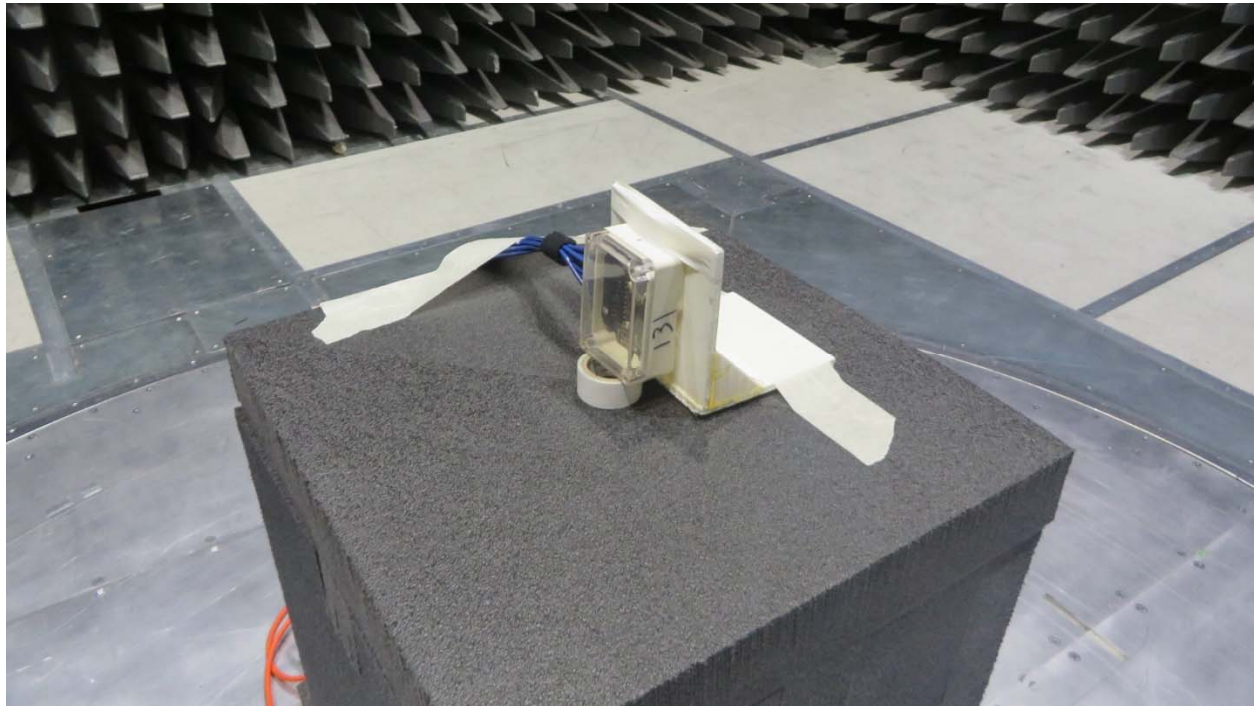
Radiated Horizontal
