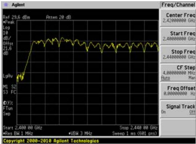
9 Channels between 2406 to 2440 MHz
