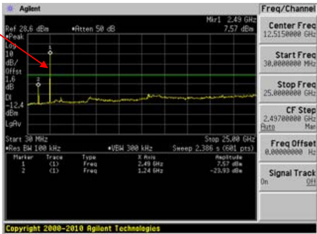
High Channel 30 MHz to 25 GHz
