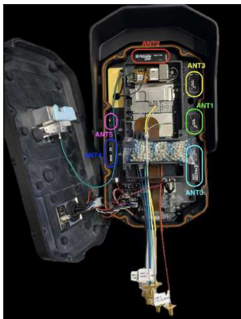
ANT0 => LTE TX/RX Main LB+MB (B2, B4, B5, B12, B13, B14, B25, B26, B66) ANT1 => LTE TX/RX Main HB (B7, B30) ANT2 => LTE RX Diversity LB (B5, B12, B13, B14, B26) ANT3 => LTE RX Diversity MB+HB (B2, B4, B7, B25, B30, B66) ANT4 => GNSS, L1 band ANT5 => Dual band 2.4GHz & 5GHz Wi-Fi/BT/BLE
