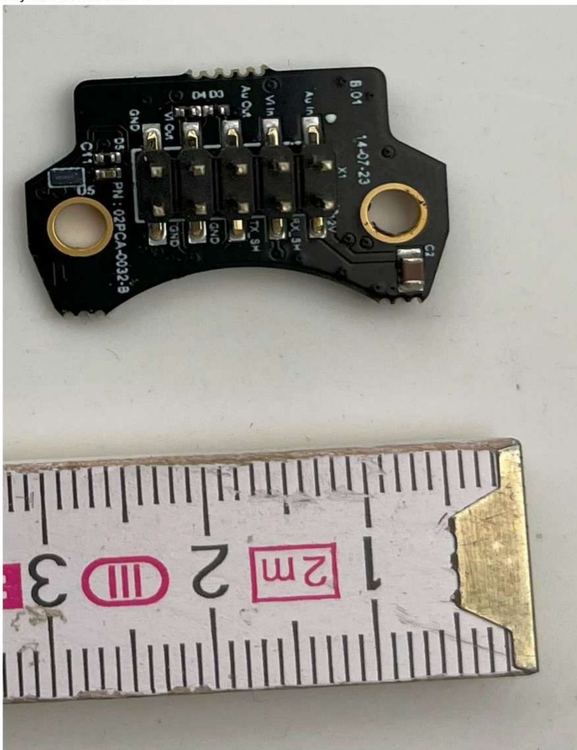
Payload connector PCBA
