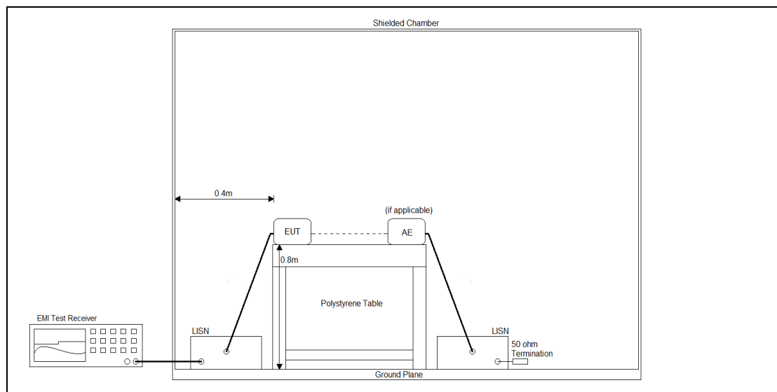
Figure 2: Test setup
