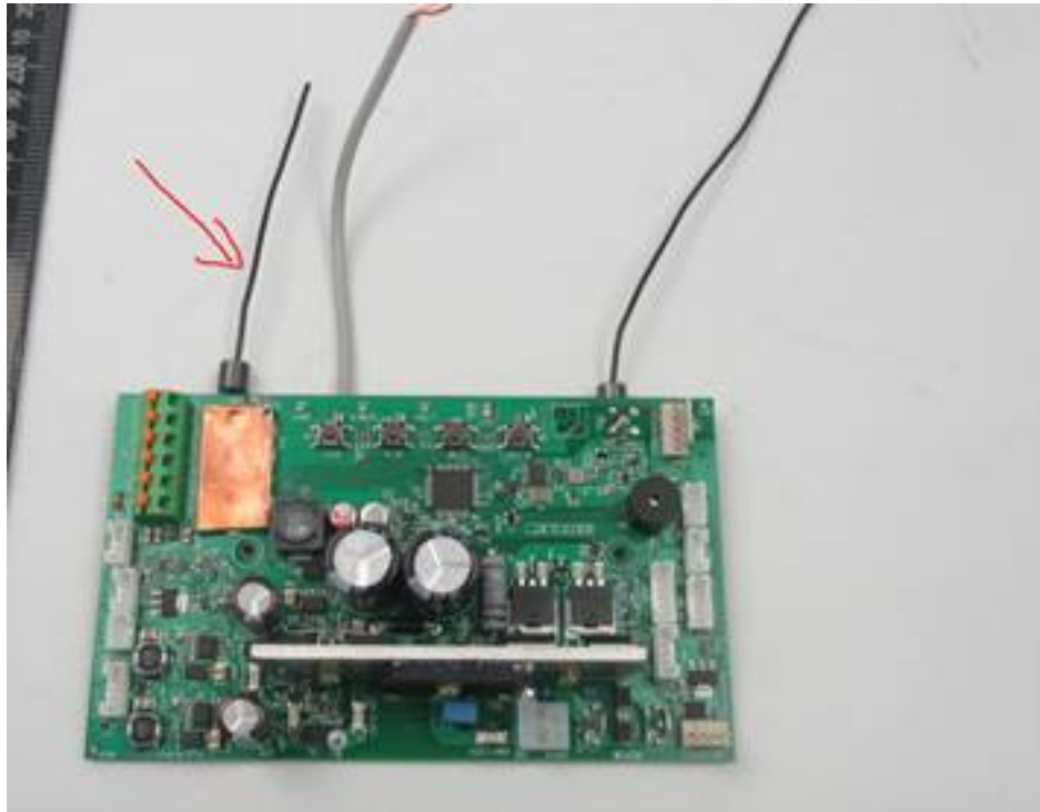
920 MHz Antenna
