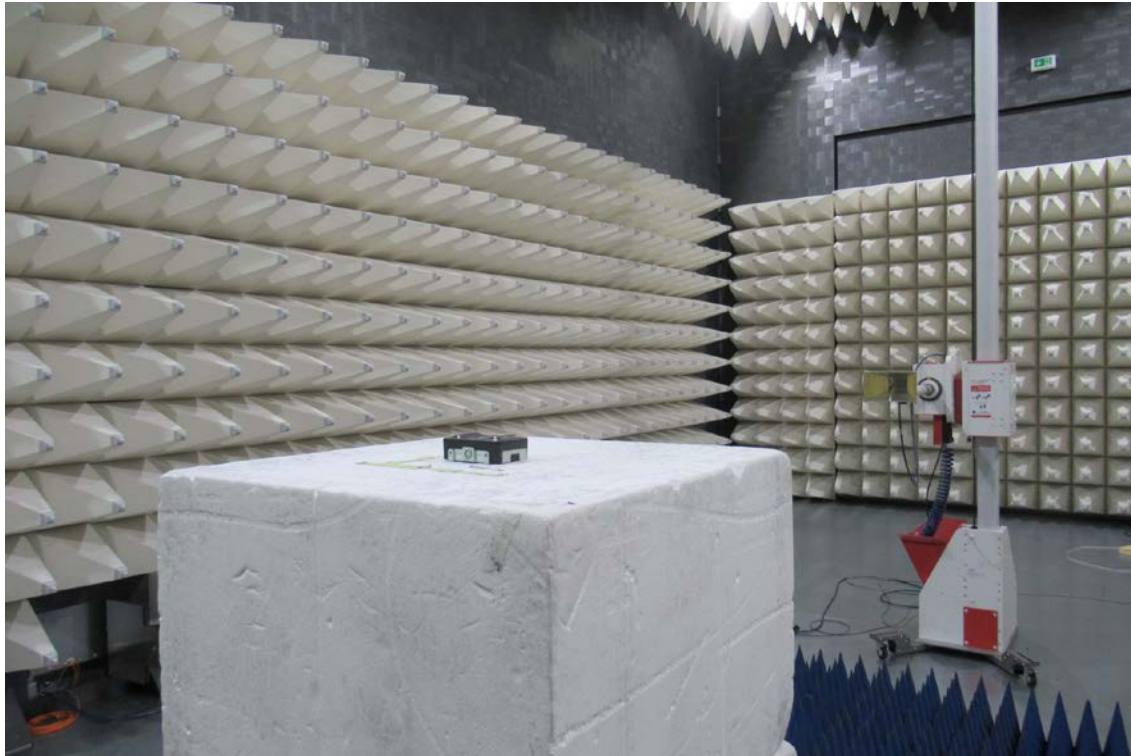
Radiated Emission (> 1000 MHz)
