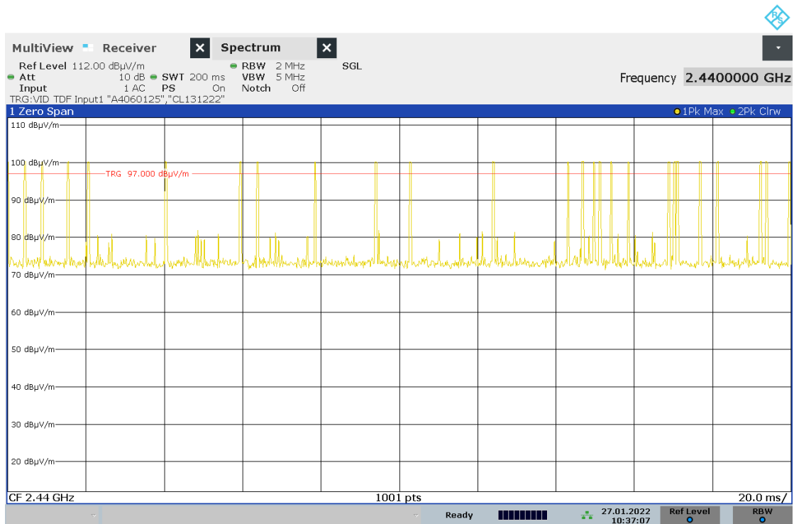
Graph 6-7: Number of hops in 0.2s period
