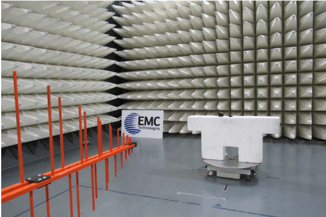
Radiated Emission (30-1000 MHz)
