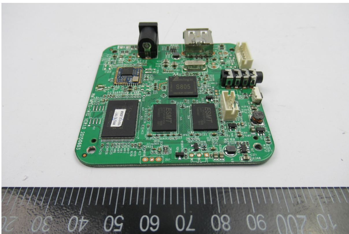
PCB Front
