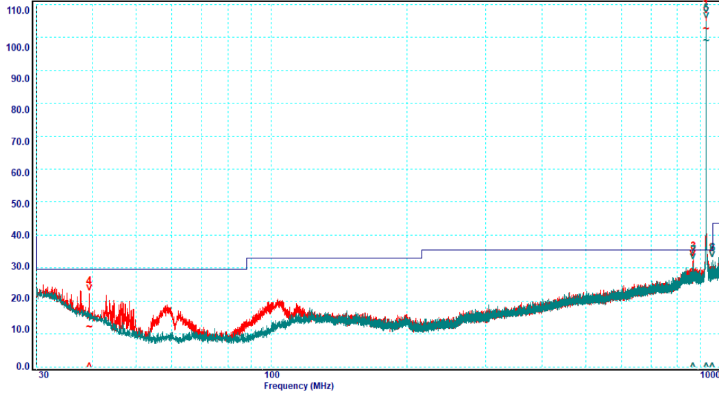
Graph 6-9: Spurious Emissions, 30 – 1000 MHz, 926.9 MHz, High Channel
