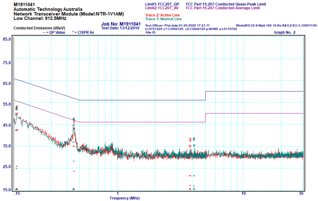
Graph 6-1: Conducted AC mains emission, 0.15 – 30 MHz, Low channel – 912.5 MHz
