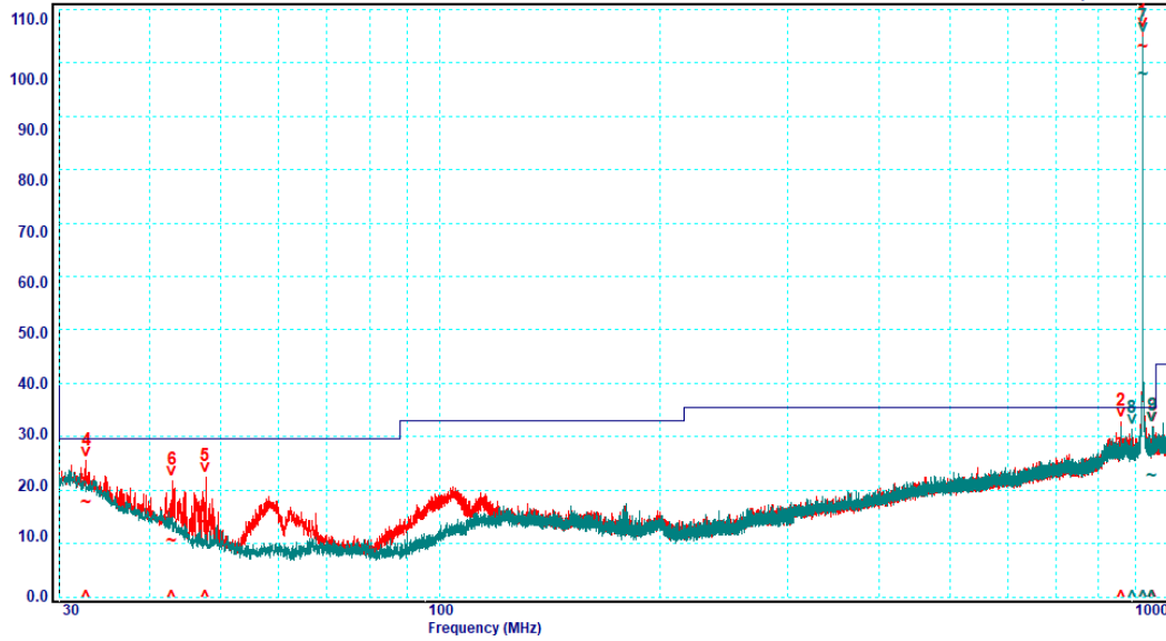
Graph 6-8: Spurious Emissions, 30 – 1000 MHz, 919.7 MHz, Mid Channel
