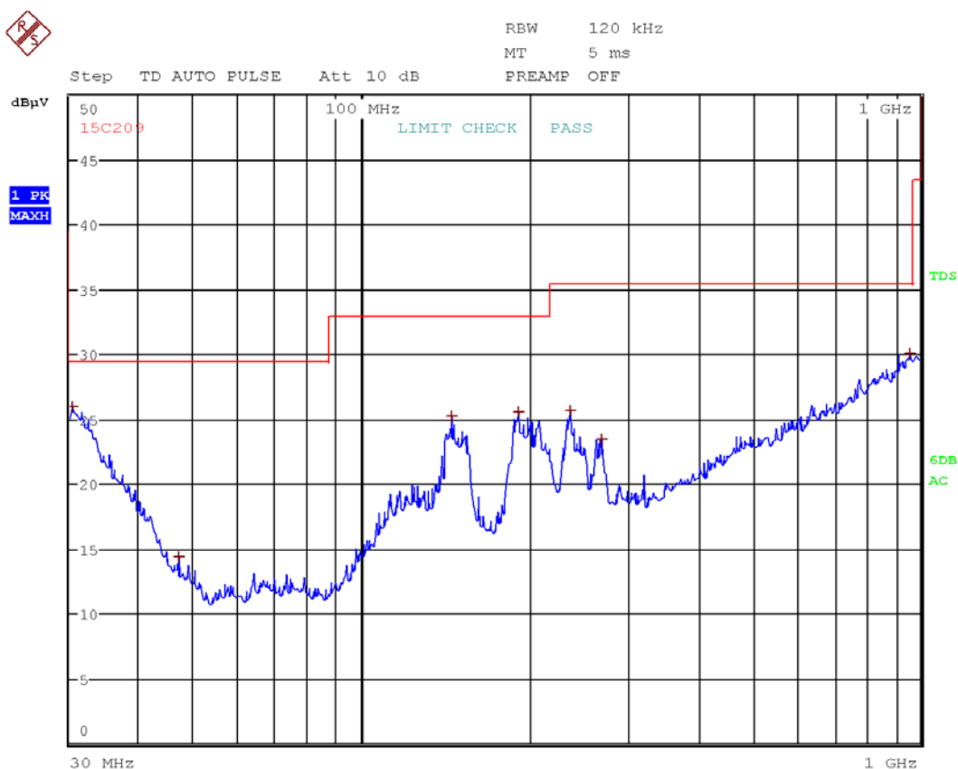
Channel 2480, Horizontal Polarisation
