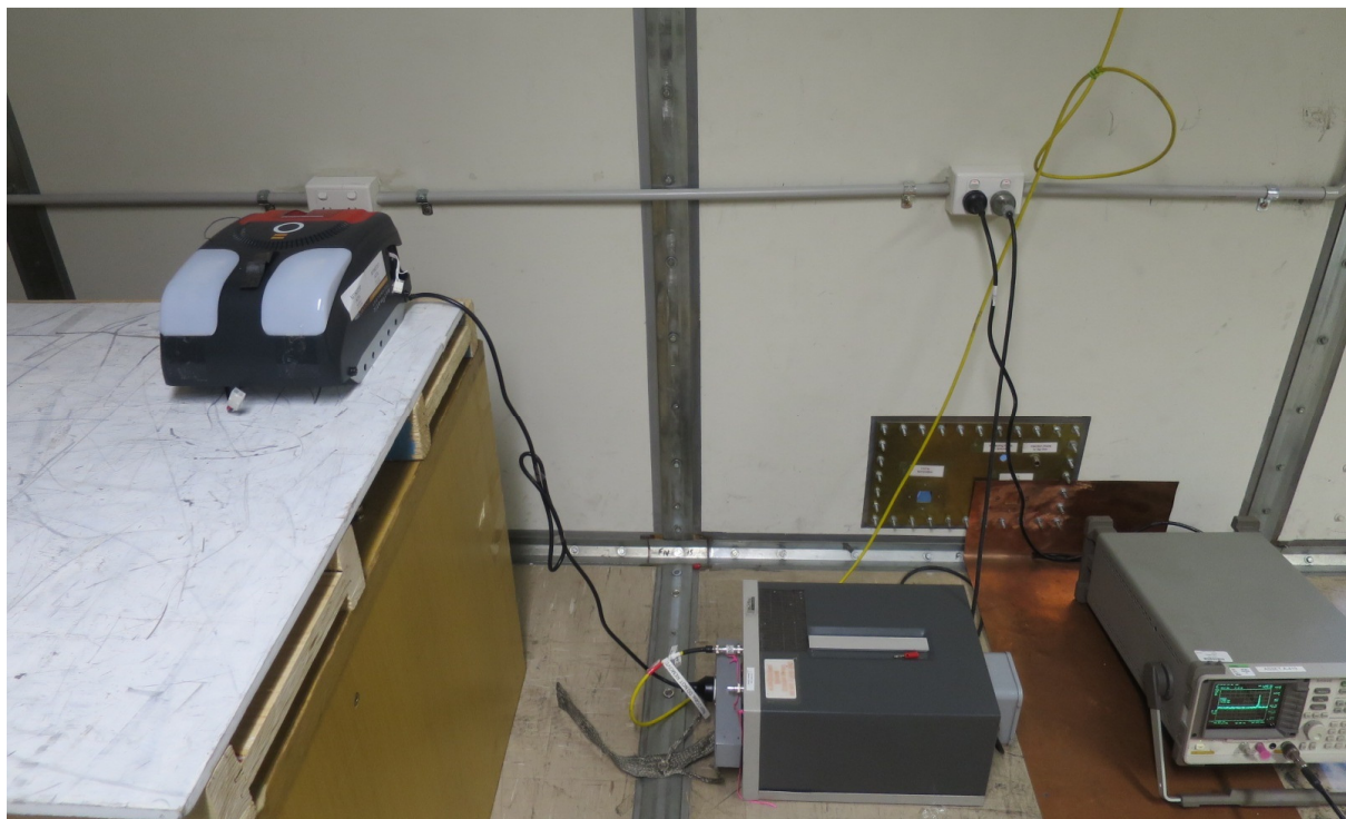
Conducted Emissions
