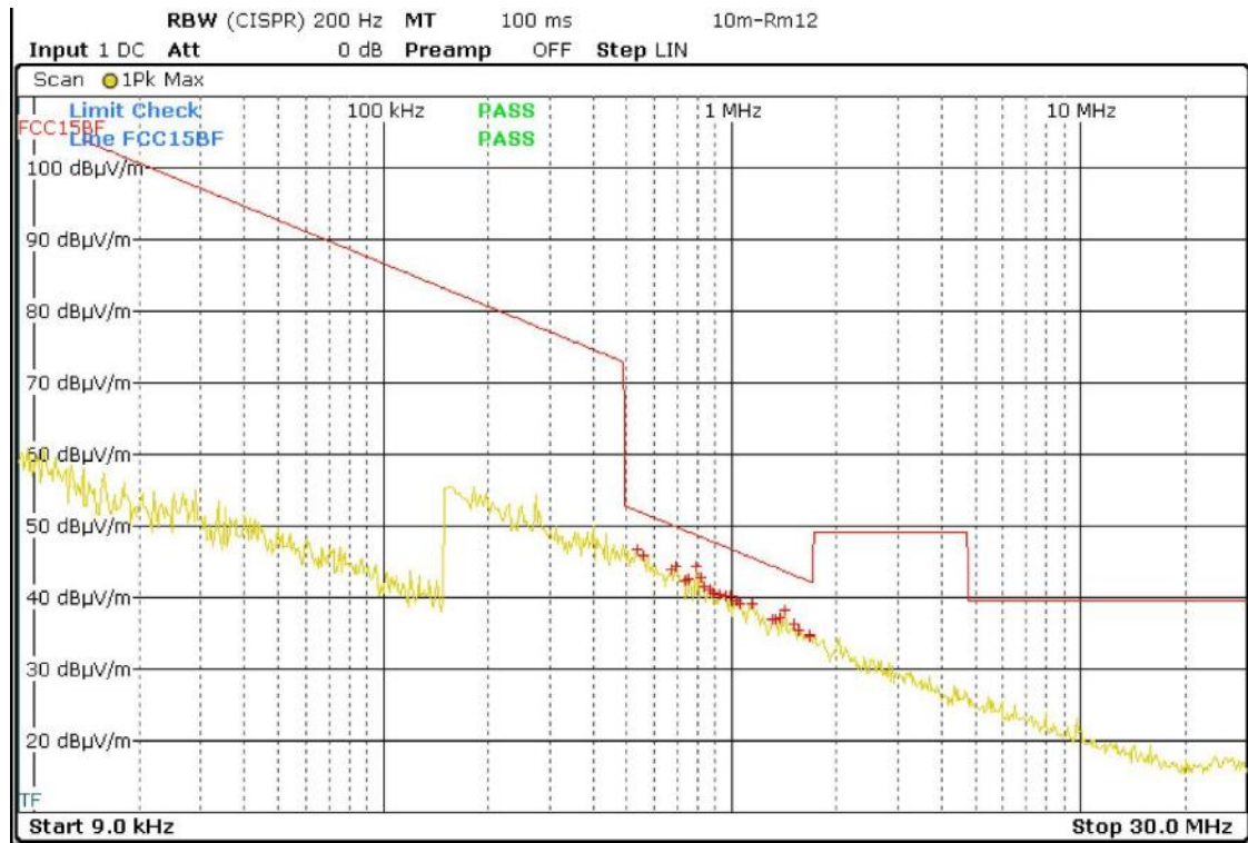
Channel 2480 MHz
