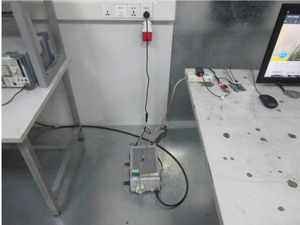
FCC ID: X4K-WSS33-1 Photo of Conducted Emission Measurement
