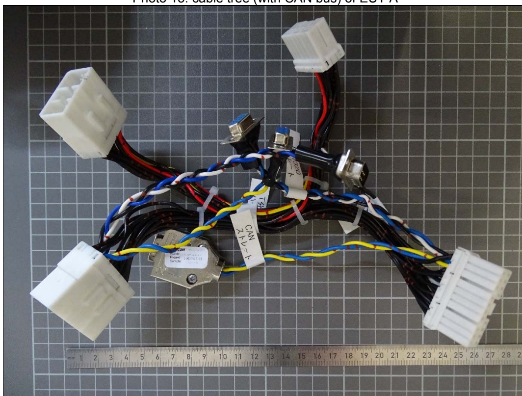
Photo 15: cable tree (with CAN bus) of EUT A
