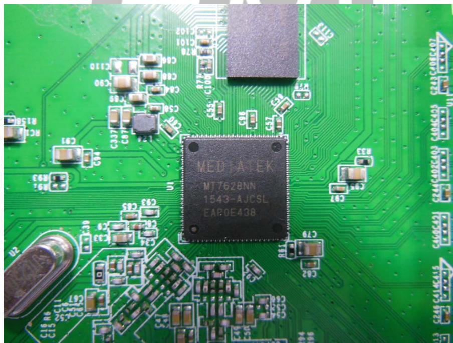
EUT –The main board View
