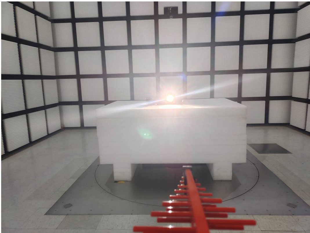
Radiated Emission Below 1GHz View (Model: AF80-NOBATT)
