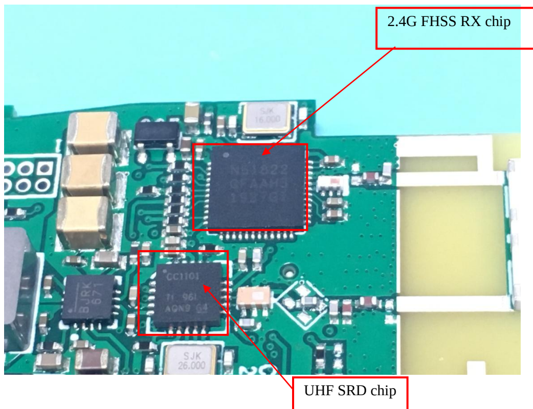
Main IC chips
